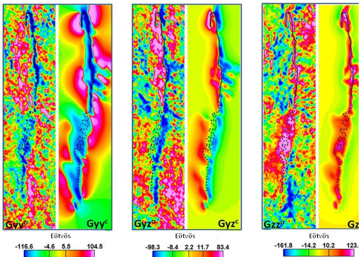
Figure 2: Observed ( G_{yy}^o , G_{yz}^o e G_{zz}^o ) and computed ( G_{yy}^c , G_{yz}^c e G_{zz}^c ) components of the gravity gradient tensor; the latter were produced by the estimated iron orebody shown in Figure 3. The black dots pinpoint the horizontal projection of the positions of the seeds specified in our inversion. All components were rotated to improve the visualization.
