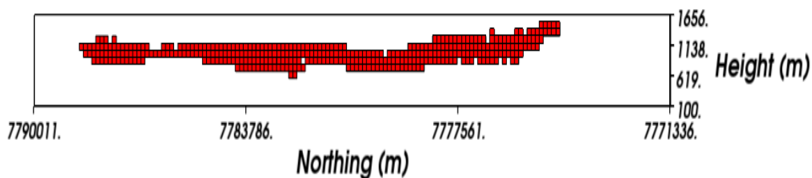
Figure 4: Quadrilátero Ferrífero iron orebody. View of the result from the eastern side. The “height” axis refers to height above the geoid. The iron orebody from the QF is shown in red prisms with density contrast of 0.5 \text{ g.cm}^{-3} .
